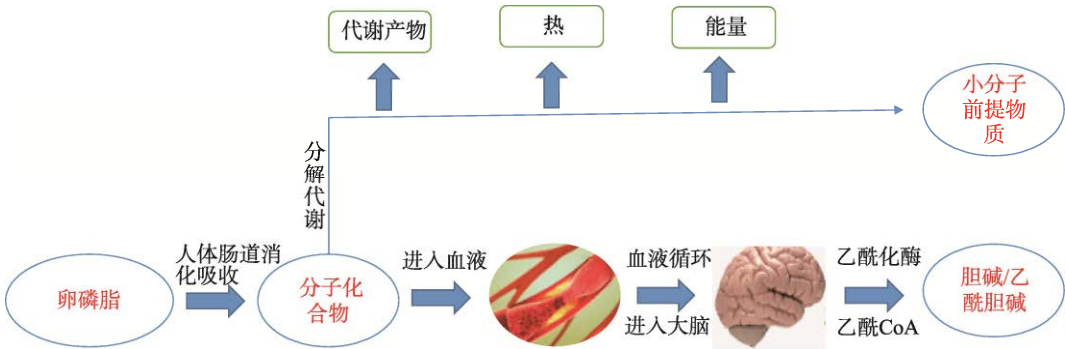
图 3 卵磷脂消化代谢路径简图 Fig.3 Diagram of PC digestive and metabolic pathways
